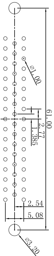
PCB layout
